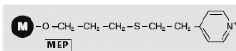
Fig. 2. Structure of the MEP Ligand (Adapted from MEP Hypercel product note).
