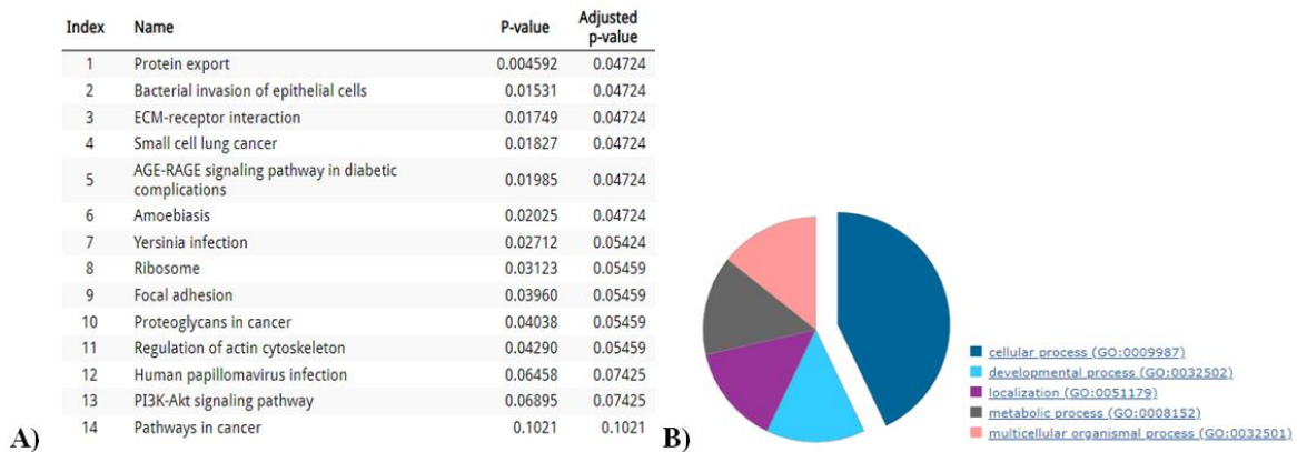
Figure 5. The image shows the functional analysis. (A) the signaling pathway of the common genes between the differentially expressed genes and the hsa-miR-508-5p target genes and (B) the biological process of the common genes between the differentially expressed genes and the hsa-miR-508-5p target genes.
