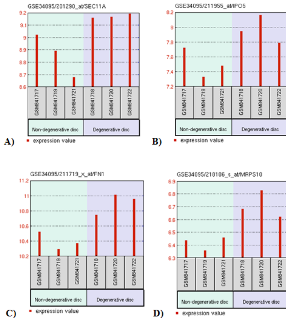
Figure 4. The image illustrates the expression levels of (A) SEC11A , (B) IPO5 , (C) FN1 , and (D) MRPS10 as the common genes among the differentially expressed genes, as well as the hsa-miR-508-5p target genes among the degenerative and nondegenerative discs samples.
