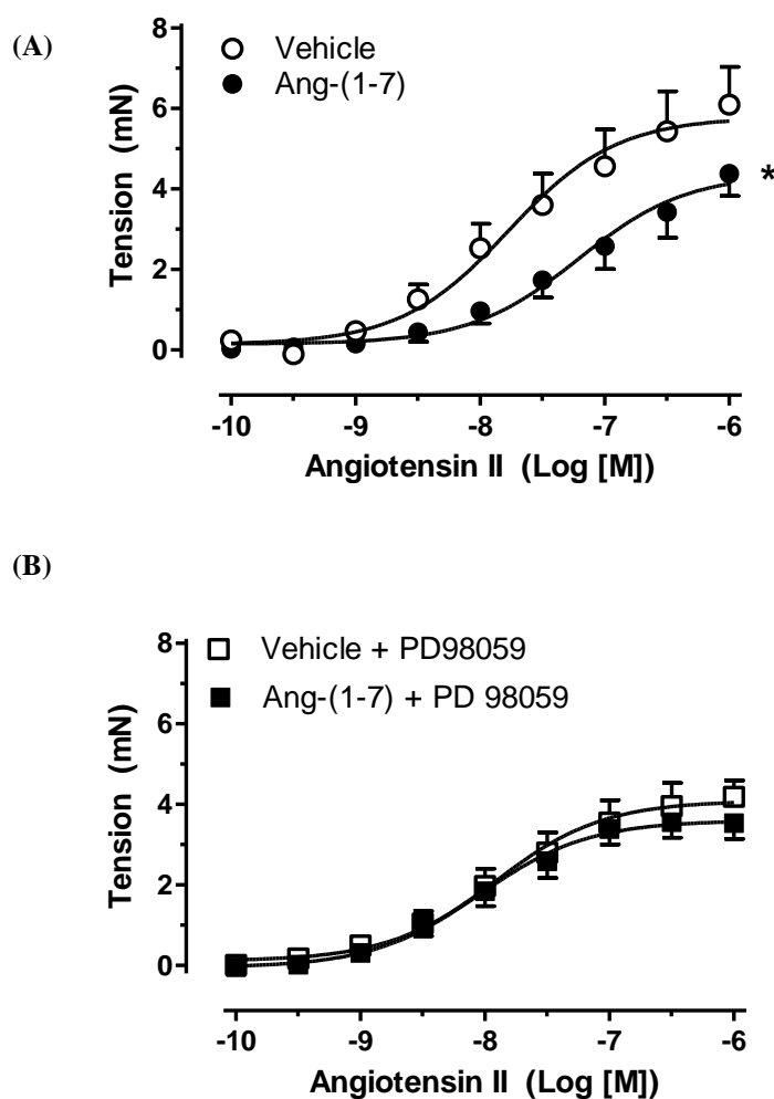
Fig.1. Ang-(1-7) decreases vasoconstriction induced by Ang II and this effect is not observed in the presence of ERK 1/2 inhibitor. A: Incubation with Ang-(1-7) (10 \mu\text{M} ), for 5 min, decreases contractions to Ang II in endothelium-denuded rat aortas vs. vehicle ( H_2O , n=8 for each group). B: ERK 1/2 inhibitor (PD98059, 10 \mu\text{M} ) abolishes differences between Ang-(1-7) and vehicle groups in contractile-response induced by Ang II. The contraction values were calculated in relation to the tension (mN), and corrected by the length (mm) of each vessel. The results are presented as mean \pm SEM for each experimental group. The statistical significance of the data was determined using the Student's t test. * P < 0.05 vs. vehicle.
