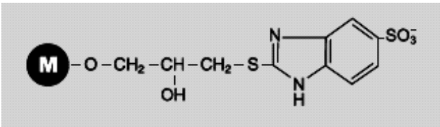
Fig. 1. Structure of the MBI Ligand (Adapted from MBI Hypercel product note). MBI ligand has a sulfonate group present on the aromatic ring.
