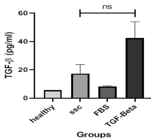
Fig. 3. TGF- \beta levels in cell culture supernatants. The differences in the TGF- \beta levels in fibroblasts, cultured with serum from healthy controls, serum from SSc patients, FBS alone and human TGF \beta 1 (10 ng/mL) + FBS, are demonstrated. Kruskal-Wallis with Dunn-Bonferroni post hoc test was used to compare the means of multiple samples. All of the experiments were repeated in duplicate for each sample. Data of each bar demonstrates means \pm SD for all values. NS: not statistically significant.
