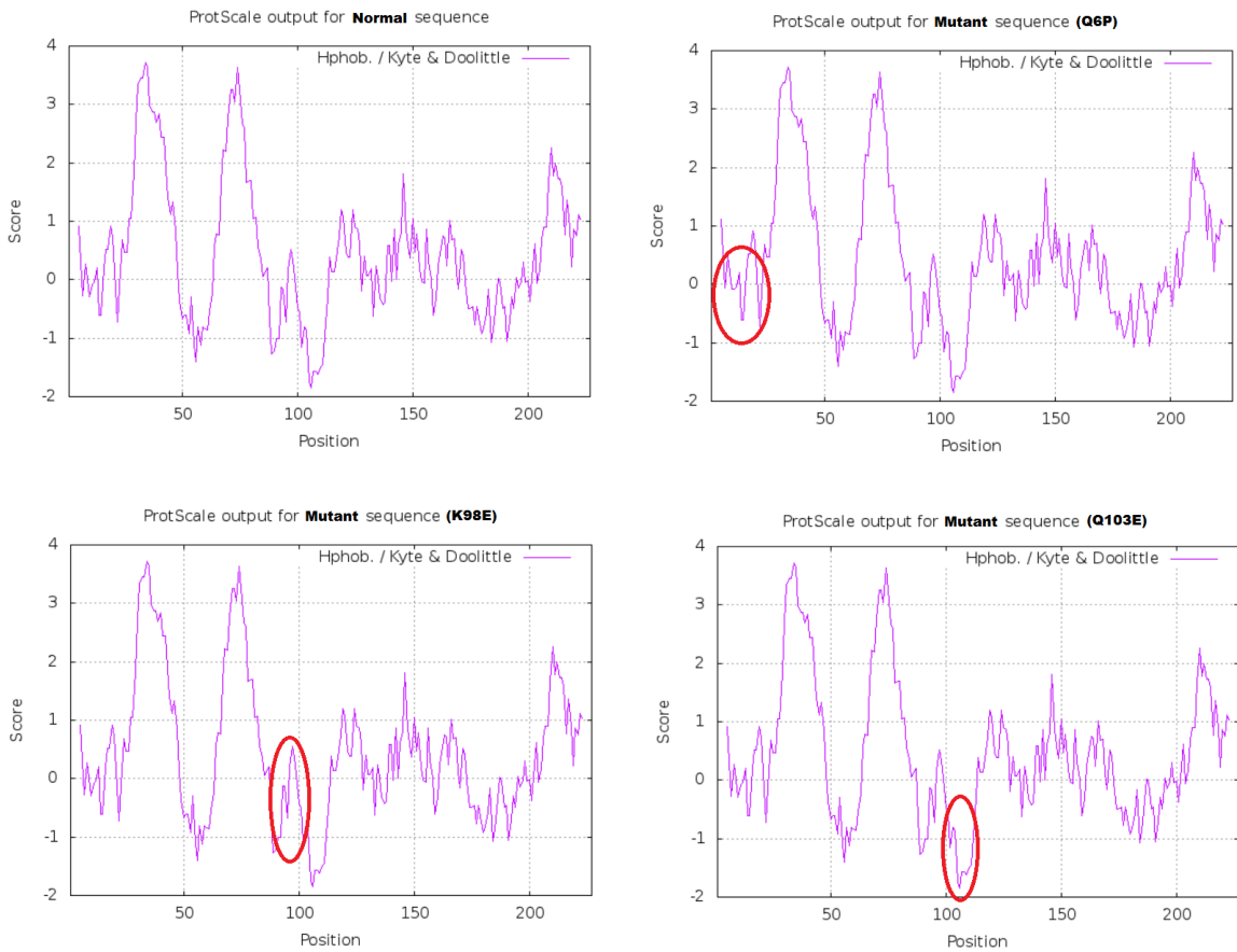
Fig. 3. Hydropathy plots for the COII subunit. The hydropobicity of the wild-type COII subunit is compared to the mutant forms for Q6P, K98E and Q103E mutations. Mutated sites are shown by circle.
