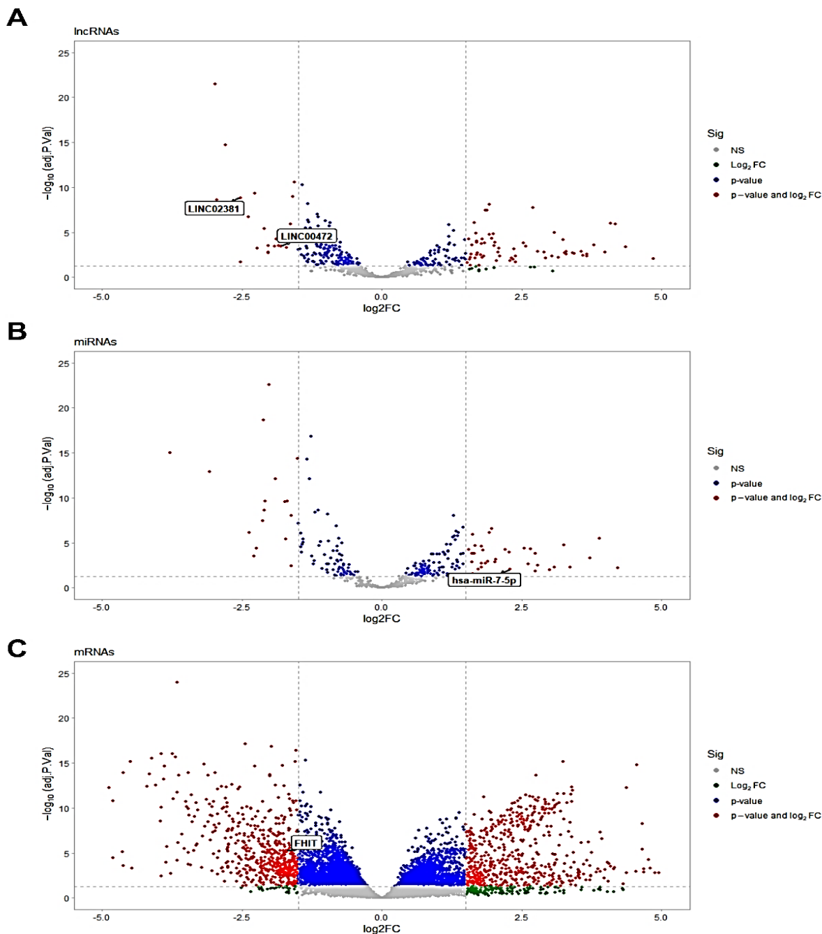
Figure 2. The volcano plot displays differentially expressed (DE) (A) lncRNAs, (B) miRNAs, and (C) mRNAs. Gray dots represent genes that did not meet either threshold ( |\log_2\text{FC}| \geq 1.5 or adjusted p < 0.05 ). Green dots indicate genes with |\log_2\text{FC}| \geq 1.5 but without statistical significance (adjusted p \geq 0.05 ). Blue dots represent
