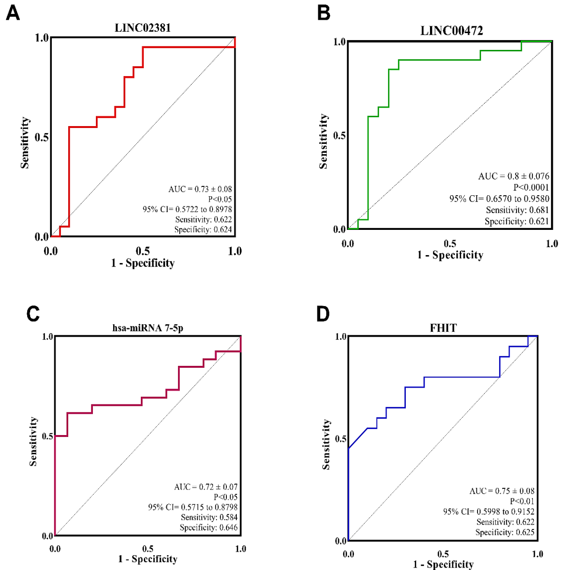
Figure 8. ROC curves were generated to assess the diagnostic accuracy of LINC02381, LINC00472, hsa-miR-7-5p, FHIT, and their combined panel in distinguishing EC tumor tissues (n = 20).
