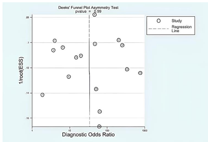
Figure 4. Deek's funnel diagram for assessing potential bias for miR-21.
