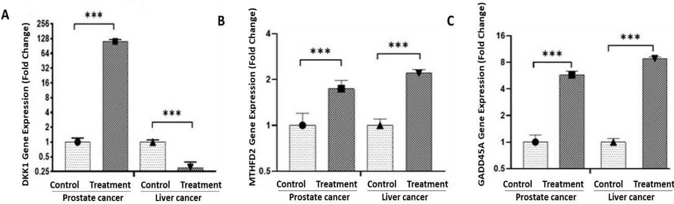
Figure 2. RNA-seq–derived expression profiles of DKK1, MTHFD2, and GADD45A following MET exposure. (A–C) Expression changes in DKK1, MTHFD2, and GADD45A derived from MET-treated prostate and liver RNA-seq datasets. MET increased DKK1 expression in prostate cells but decreased it in liver cells, while MTHFD2 and GADD45A were consistently upregulated in both datasets. Statistical significance was based on DESeq2 FDR-adjusted p -values (*** p_{adj} < 0.0001 ).
