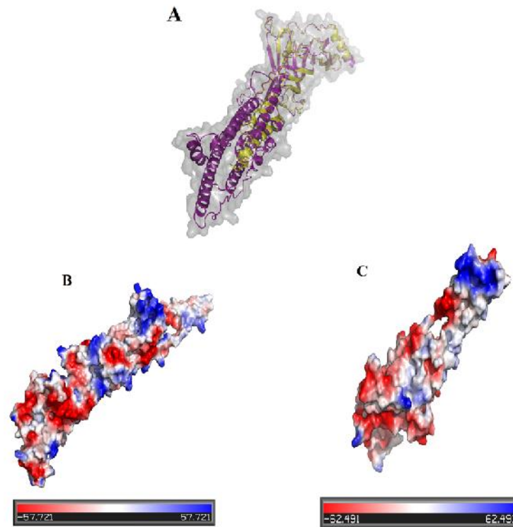
Fig. 5. Predicted structure of native and truncated protein. (A) Superimposition of the best predicted models of native and truncated protein. The native protein structure was shown in magenta and truncated protein in yellow. Surface electrostatic potential of native protein (B) and mutant proteins (C); blue, red and white colors represent the positive, negative and hydrophobic regions, respectively.
