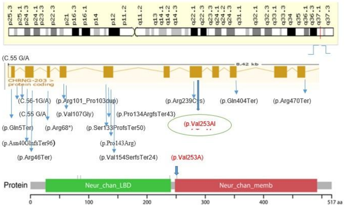
Fig. 6. Schematic representation for localization of the identified CHRN2 variants in neurotransmitter-gated ion-channel transmembrane region.
